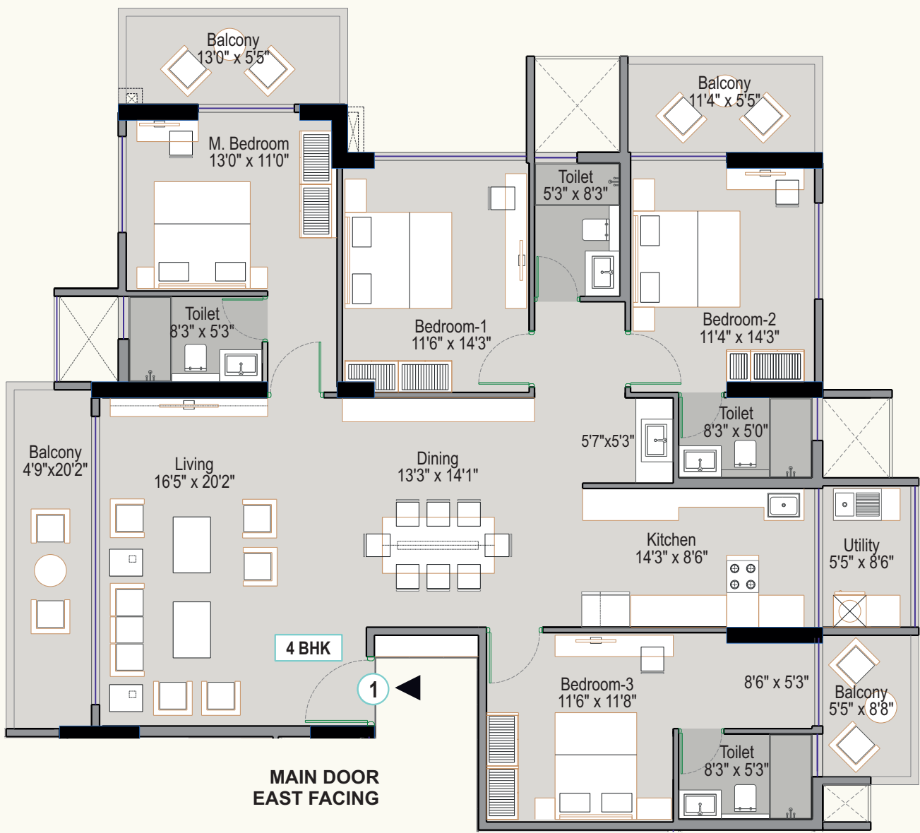
FLOOR PLAN
